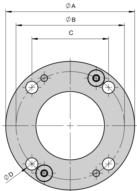
FC Flange
