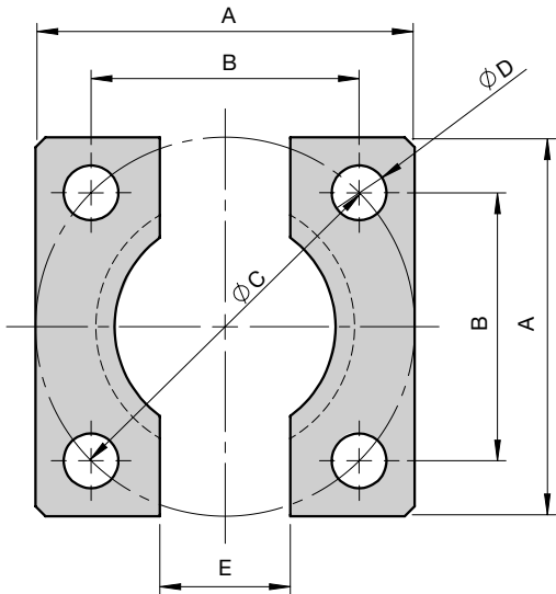
FFCX Flange
