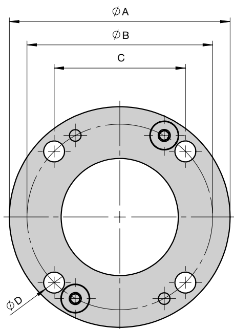
FCN Flange
