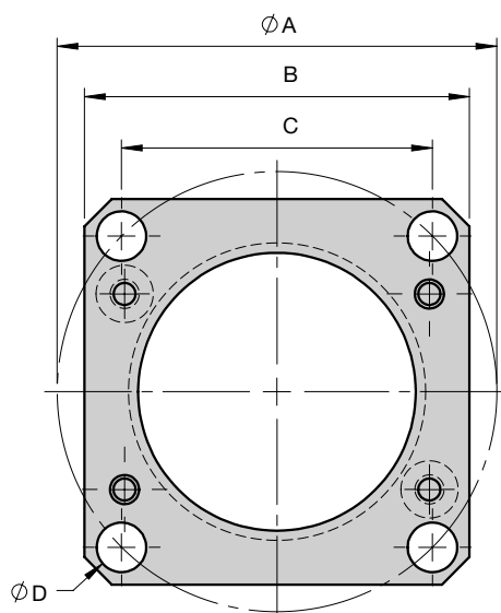
FCX Flange
