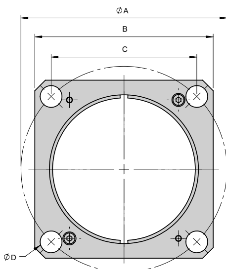
FK Flange
