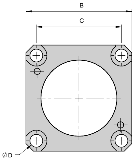
FCSC Flange
