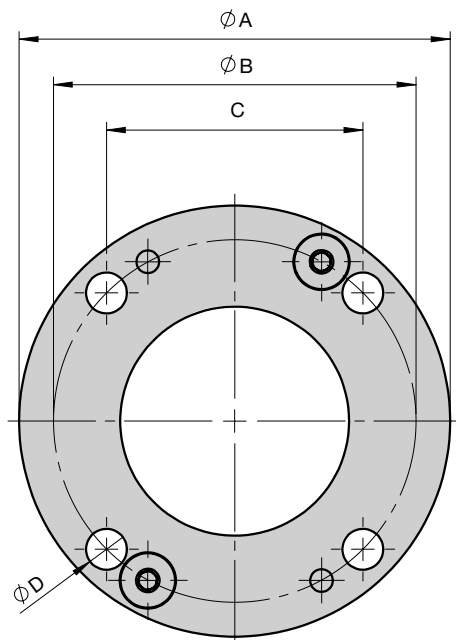
FCN Flange
