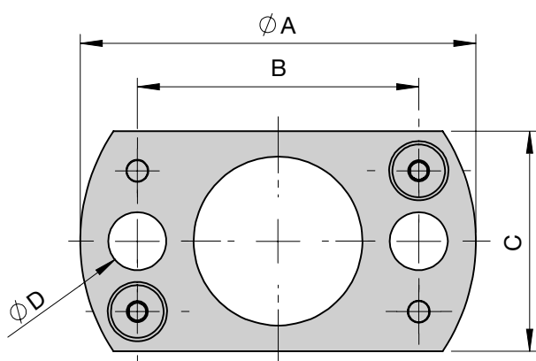
FCR Flange
